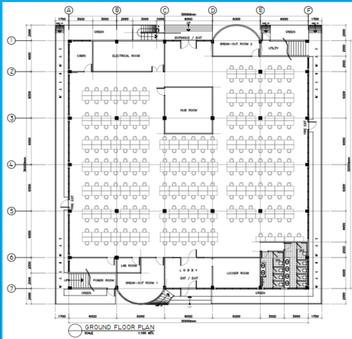
GROUND FLOOR PLAN 1,000 sqm.
