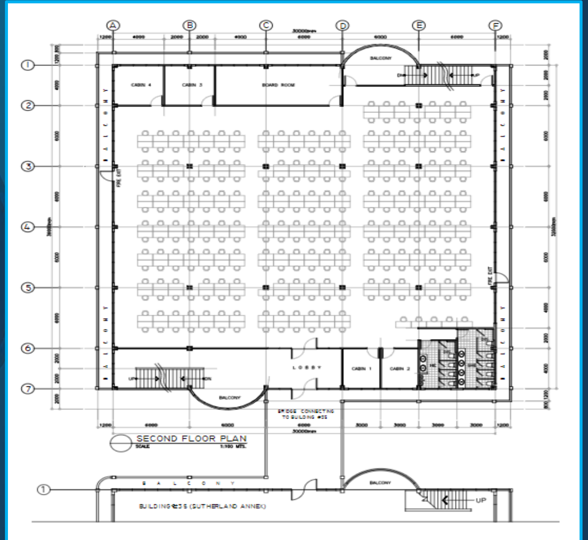
SECOND FLOOR PLAN 1,000 sqm.
